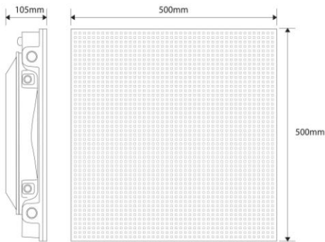
Cabinet dimension
